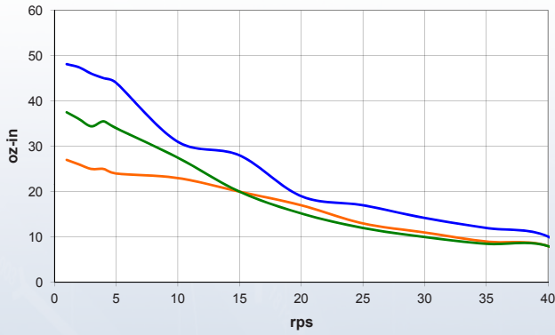
HT23 with STR4
