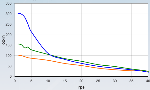
HT34 with STR8
