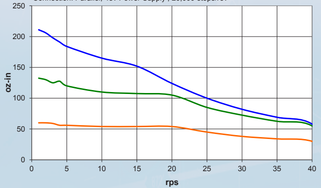
HT24 with STR8
