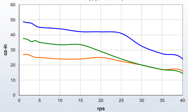
HT17 with STR4
