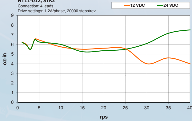
STR2 24V, Connection: Parallel 20000 steps/rev
