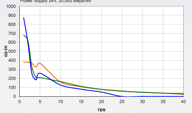
HT34 with STR8
