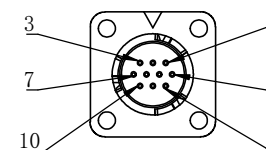
Encoder Connector: XM10-S10S-C(EUMACX)
