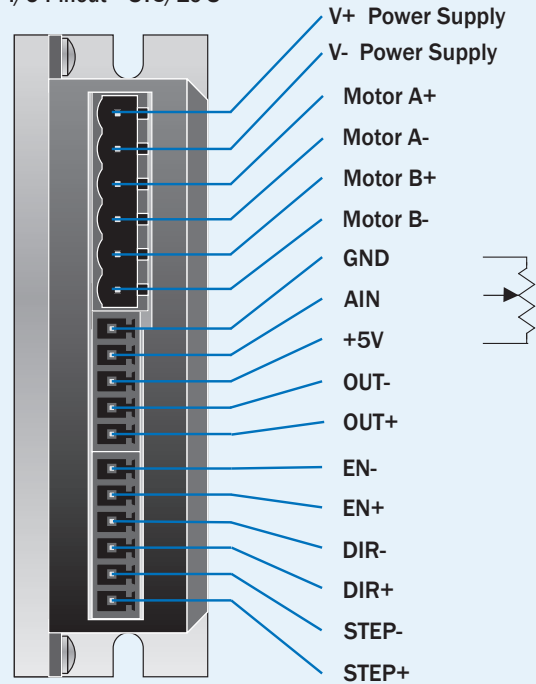
I/O Pinout - ST5/10-S
